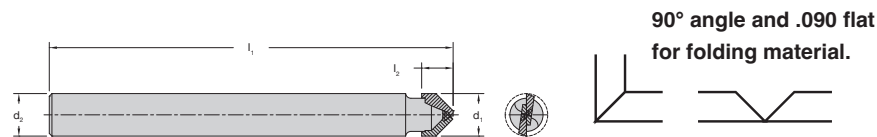
37-70 Series Two Flute - V Bottom Carbide Tipped Product Offering
