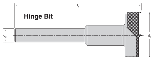
72-000 Series Carbide Tipped Hinge Bit Product Offering - Metric
