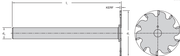
70-300 Series Solid Carbide Tipped Trim Blade Flush Mount Product Offering
