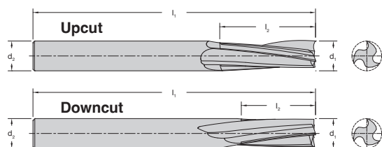
60-200 Series Three Flute - Solid Carbide Low Helix Finisher Upcut Product Offering
