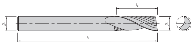
65-100 Series Single Flute - Solid Carbide Upcut O Flute Product Offering
