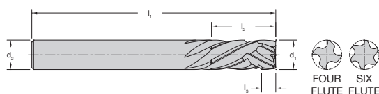
66-800 Series DFC Compression Product Offering
