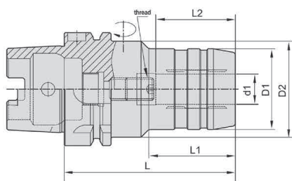
34-170 Series HSK63F Hydraulic Holders
