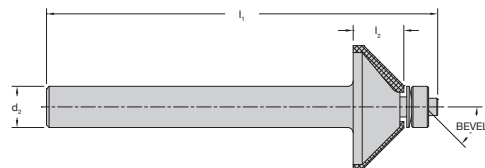
29-50 Series Two Flute Carbide Tipped Chamfer Product Offering
