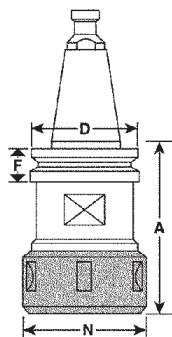
33-70 Series ISO Toolholders for CNC Routers Product Offering
