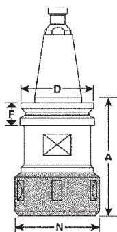
33-80 Series BT Toolholders for CNC Routers Product Offering
