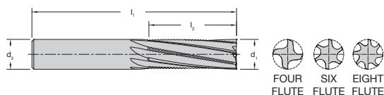
66-775 Series DFC Low Helix Rougher Finisher Upcut Product Offering
