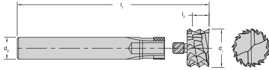
34-000 Series Solid Carbide Aircraft Panel Tools Product Offering
