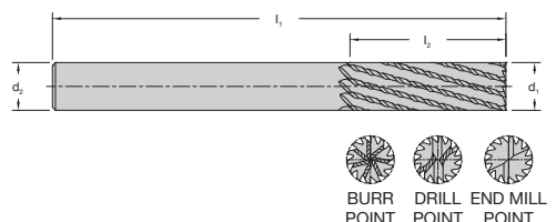
66-500 Series DFC Multi-Flute Composite Router Product Offering
