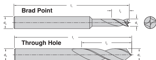
72-000 Series Solid Carbide Boring Bits Brad Point - Right Hand Rotation Product Offering - Metric
