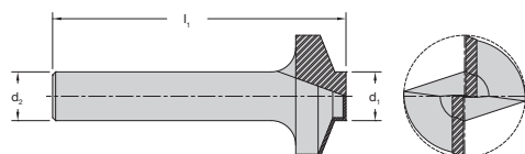
47-00 Series Two Flute - Carbide Tipped MDF Panel Tools Product Offering
